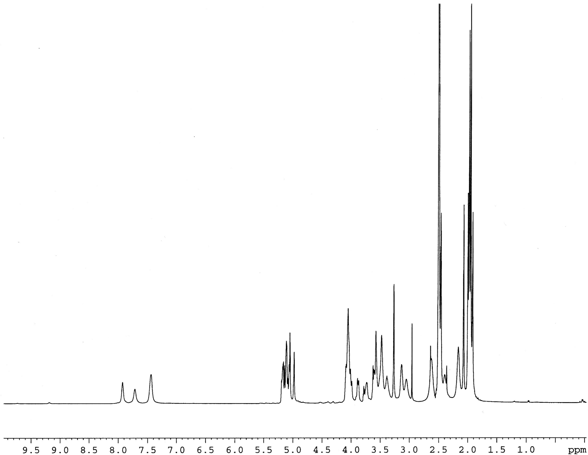
Figure S2. 1 H NMR spectrum (500 MHz, d 6 -DMSO) of 8.
