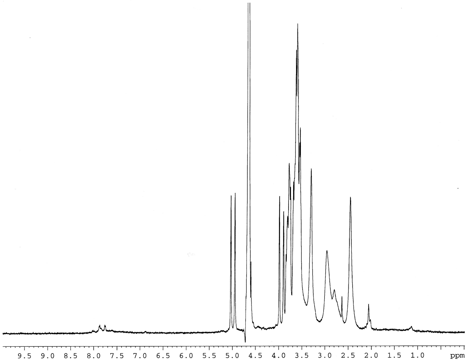
Figure S4. 1 H NMR spectrum (500 MHz, d 6 -DMSO) of 10.
