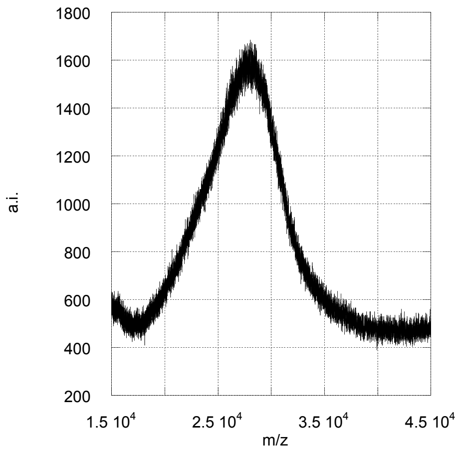
Figure S5. Unsmoothed MALDI spectrum of 7 .
