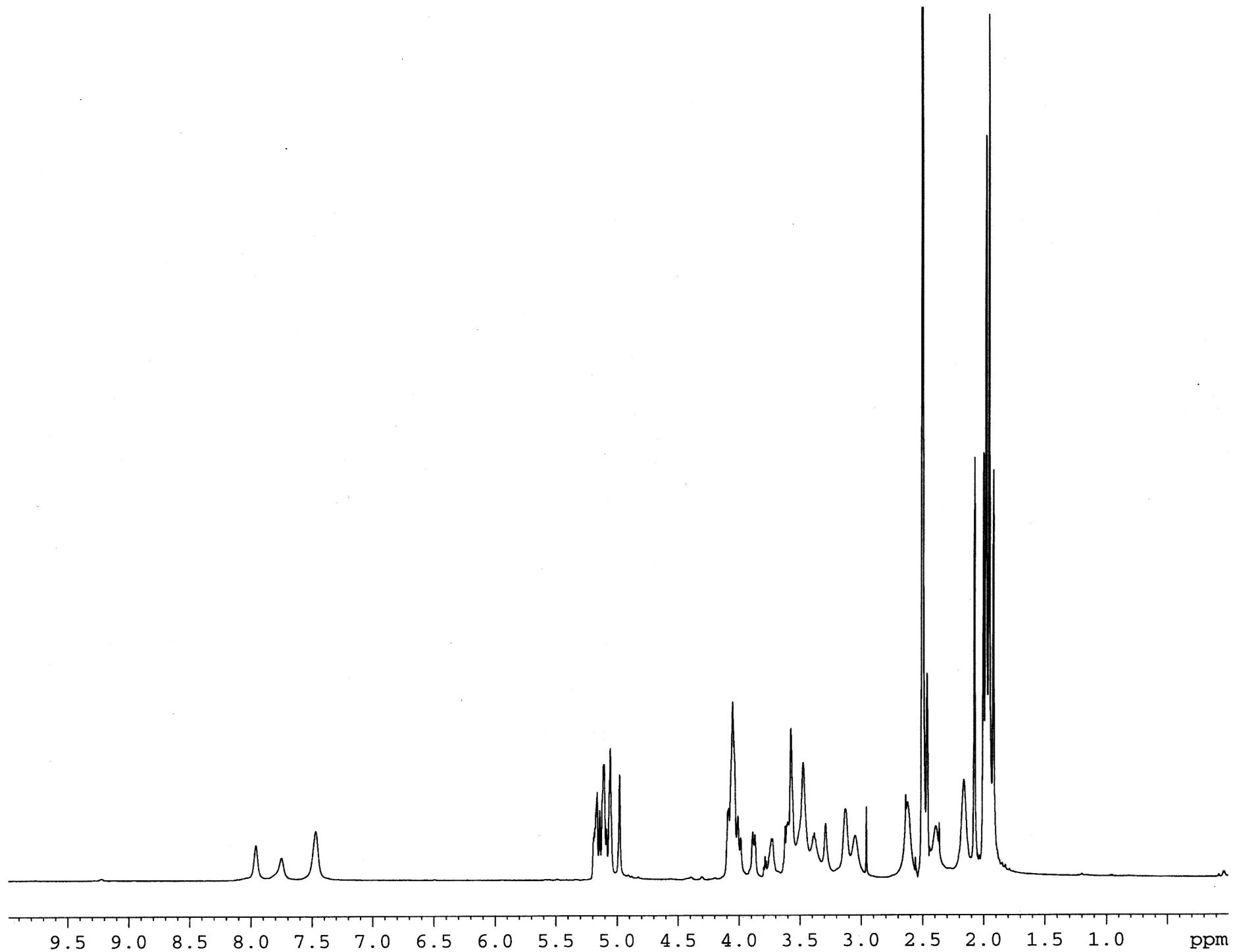
Figure S1. 1 H NMR spectrum (500 MHz, d 6 -DMSO) of 7.
