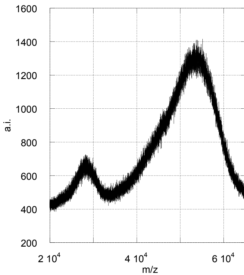
Figure S6. Unsmoothed MALDI spectrum of 8 .
