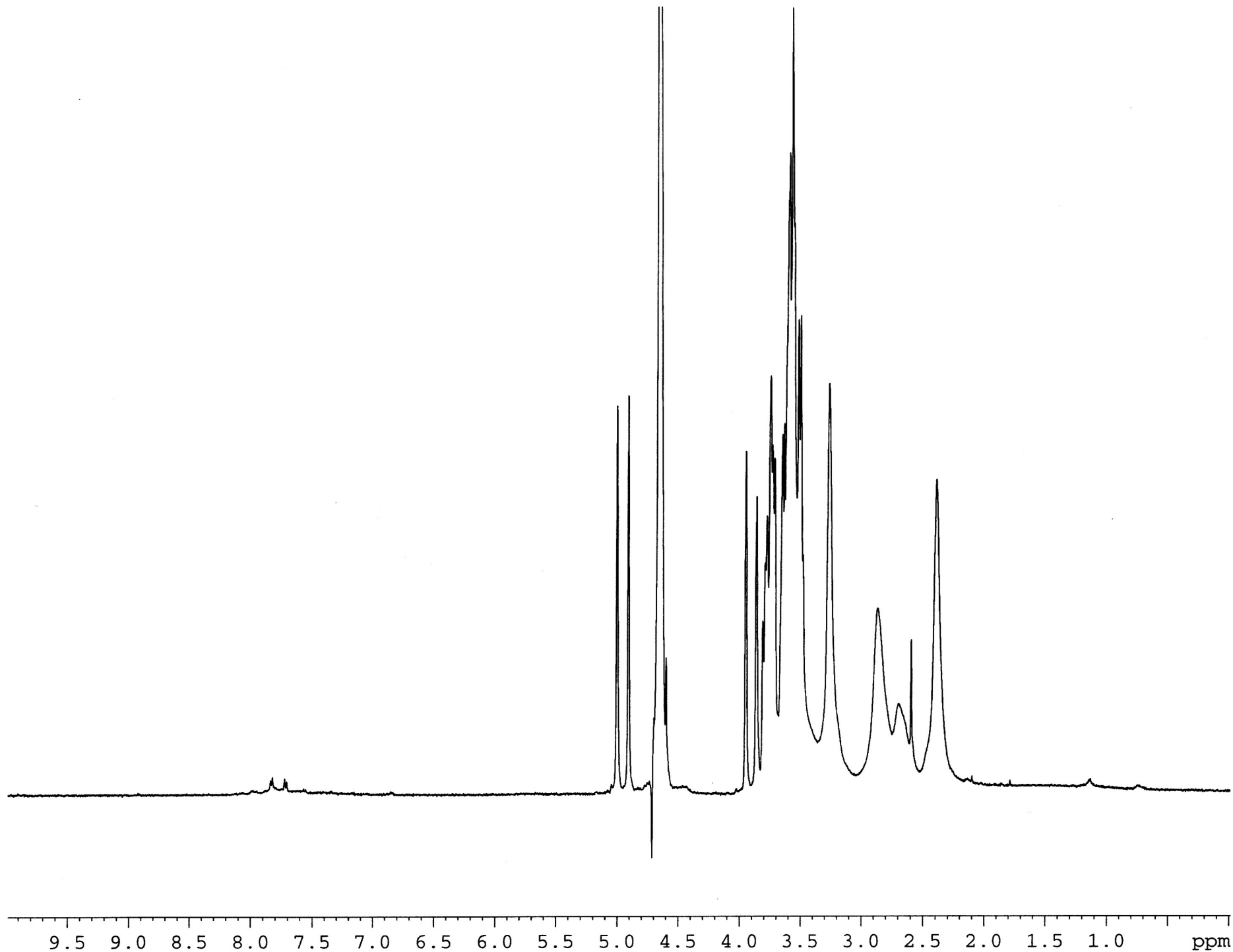
Figure S3. 1 H NMR spectrum (500 MHz, d 6 -DMSO) of 9.
